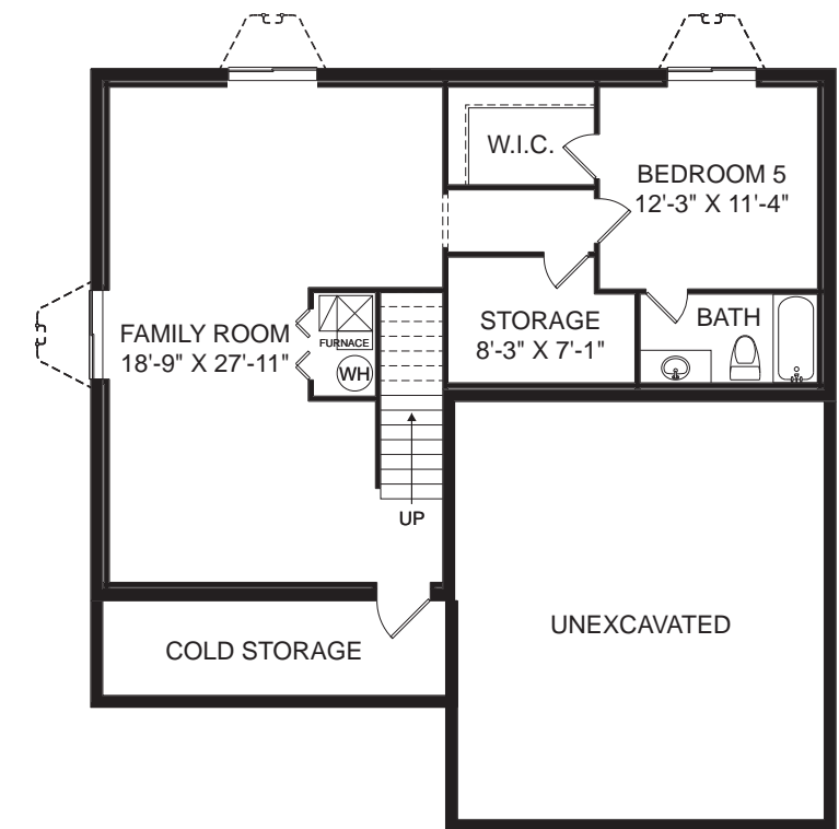
Optional Finished Basement - Fully Finished
